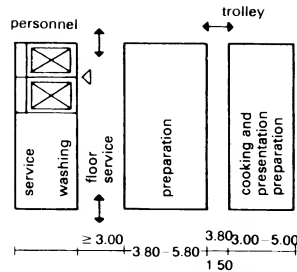
2 Layout for medium-size/large businesses
